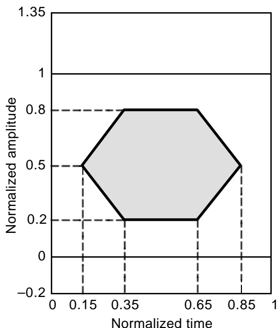
Figure 3 – Transmitter eye diagram mask
