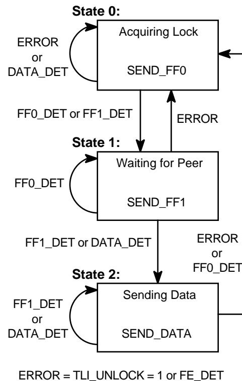
Figure 2 – Link reset state diagram
