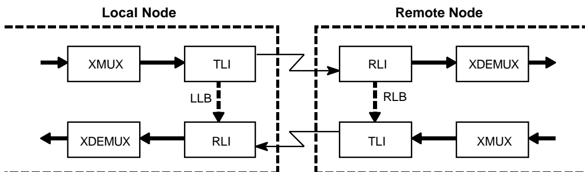
Figure D.1 – Remote and local loopback
