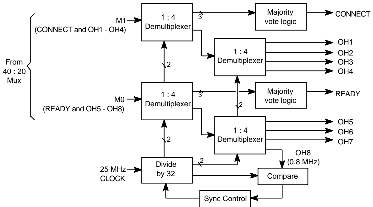
Figure A.2 – SUBDEMUX block diagram
