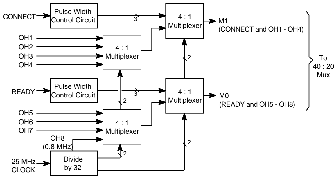
Figure A.1 – SUBMUX block diagram
