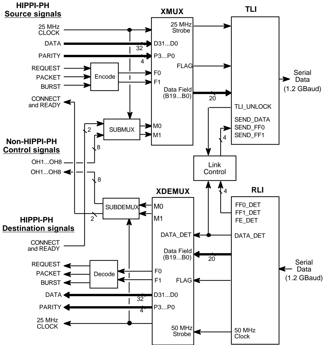
Figure 1 – 32-bit, dual-simplex, HIPPI-Serial functional units example
